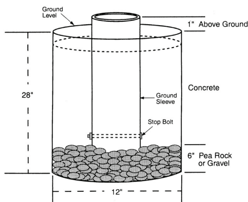
Hole Diagram
